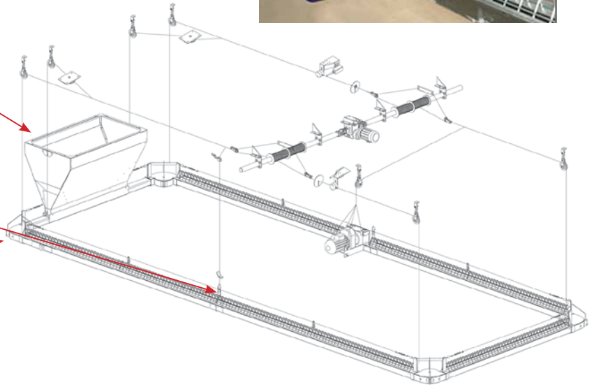
Drive unit for suspended chain feeding system
