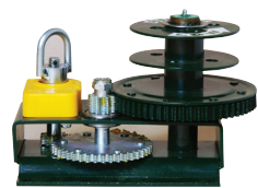
Winch 1350 kg For pan feeding over 60 m
