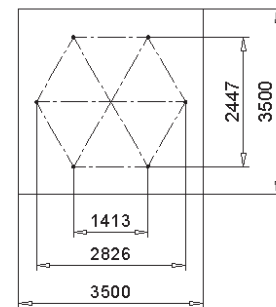
Base concrete drawing for 6-leg silos
