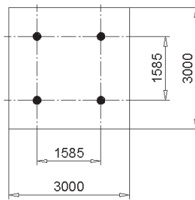
Base concrete drawing for 4-leg silos
